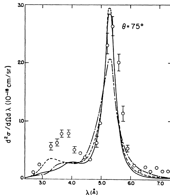
FIG. 8. Same as Fig. 7 for \theta = 75^\circ .
