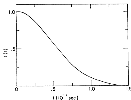
FIG. 2. f(t) as a function of time using Eq. (34). The values of c and \alpha are as cited in the text and \delta^2 = 3.0 \times 10^{26} / \text{sec}^2 .
