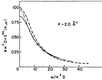
FIG. 3. \pi \kappa^2 D S^{\text{inc}}(\kappa, \omega) as a function of \omega / \kappa^2 D for \kappa = 2.0 \text{ \AA}^{-1} . Computed for argon at T = 85.5^\circ \text{K} using D = 1.88 \times 10^{-6} \text{ cm}^2/\text{sec} . The Gaussian results obtained by Nijboer and Rahman, Ref. 36 (—) are compared with the results obtained as described in the text (---), and the exact results (- · -) from Ref. 36.
