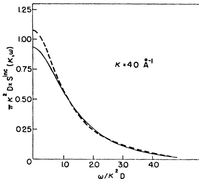
FIG. 4. \pi \kappa^2 D S^{\text{inc}}(\kappa, \omega) as a function of \omega / \kappa^2 D for \kappa = 4.0 \text{ \AA}^{-1} computed for argon at T = 85.5^\circ \text{K} using D = 1.88 \times 10^{-6} \text{ cm}^2/\text{sec} . The Gaussian results obtained by Nijboer and Rahman, Ref. 36 (—) are compared with the results obtained as described in the text (---).
